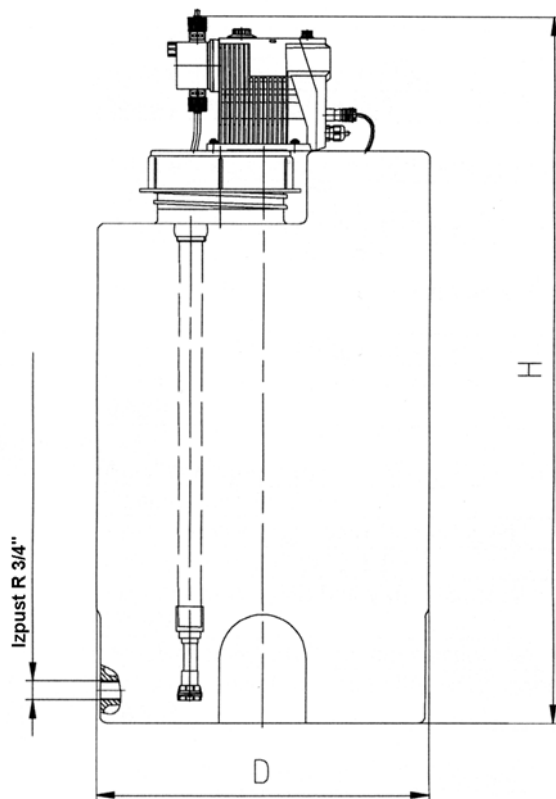
Dosing station DP
